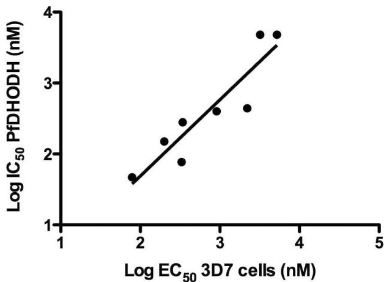
Figure 4. Comparison of the series activity on PfDHODH vs P. falciparum whole cell assays. The log of the PfDHODH IC 50 data are plotted versus the log of the P. falciparum EC 50 data (in nanomolar). The plotted data include compounds 1 , 2 , 4–16 described in the Table 1. Compounds for which solubility limits prevented the quantitative determination of either the IC 50 or EC 50 have been left off the plot. Data were fitted by linear regression analysis where r^2 = 0.84 and slope = 0.93.
