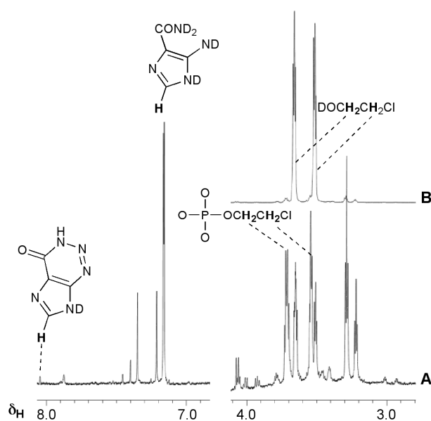
Figure 2. Reaction of MTZ with phosphate buffer pD = 7.8, 37 °C. (A) ^1\text{H} -NMR spectrum after 14 days; (B) The same sample spiked with authentic chloroethanol ( 7 ).
