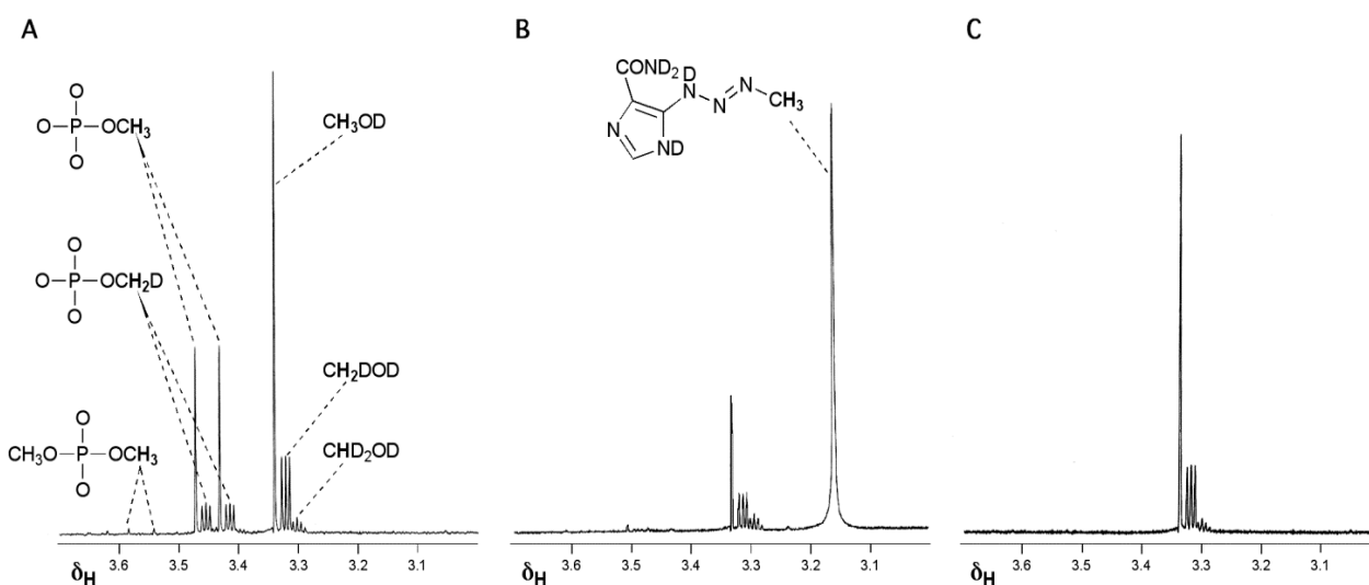
Figure 1. Reaction of TMZ, MTIC and \text{CH}_2\text{N}_2 in \text{D}_2\text{O} systems. (A) Products of reaction of TMZ with phosphate buffer pD = 7.8 showing deuterium incorporation into methanol and methyl phosphate; (B) MTIC in \text{Na}_2\text{CO}_3 (10% in \text{D}_2\text{O} ) showing the intact isotopic configuration of the MTIC methyl and deuterium incorporation into the methanol product of hydrolysis; (C) Products of condensing diazomethane into \text{Na}_2\text{CO}_3 (10% in \text{D}_2\text{O} ) [15–17].
